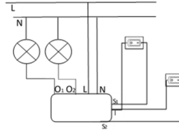
Figure 1 Diagram for connecting the device
